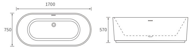
STRIATA FLOORSTANDING BATH
